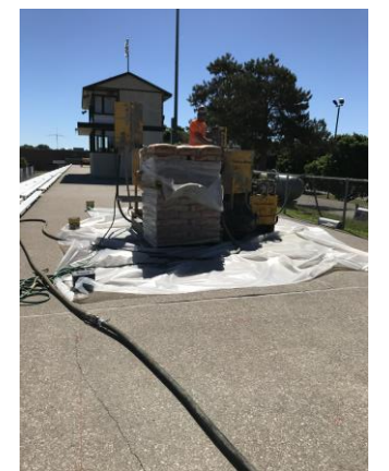
Grout pump at Midland High Football Stadium
